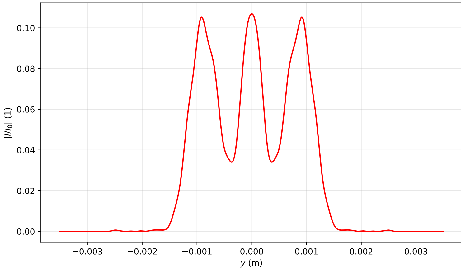
Intensity profile I(x=0, y, z=2.388)/I_0 , P_{in}=7.5P_{cr} , artificial time
